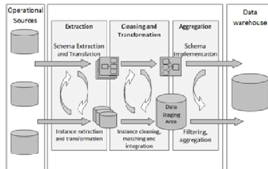
Fig 2. Extraction, Cleaning, Transformation and Loading Process.
