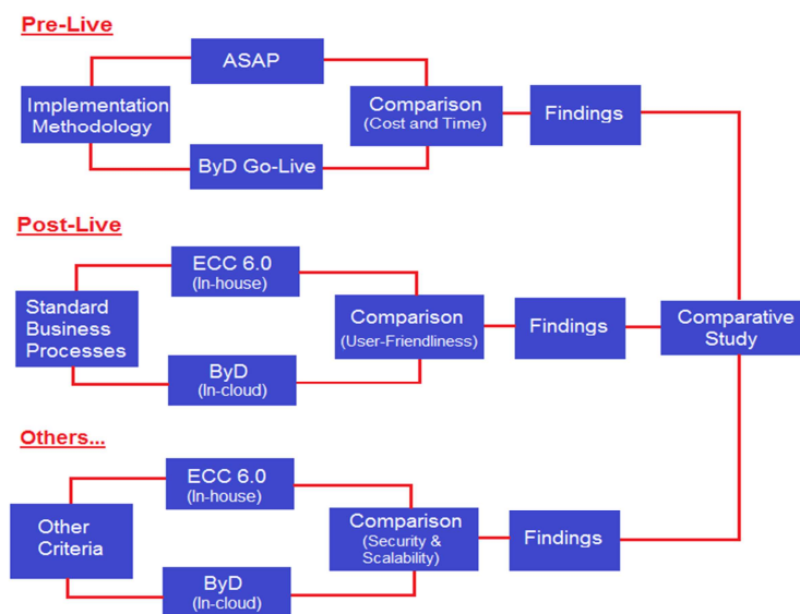
Figure 2. Methodology Diagram
