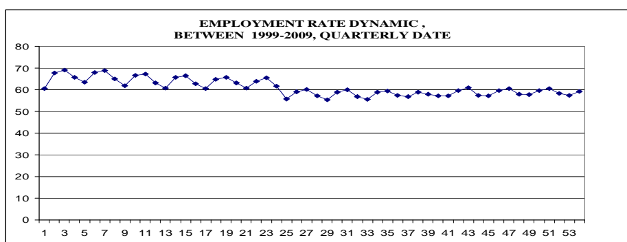
Fig 1. Employment Rate Dynamic between 1999-2009, in Romania
