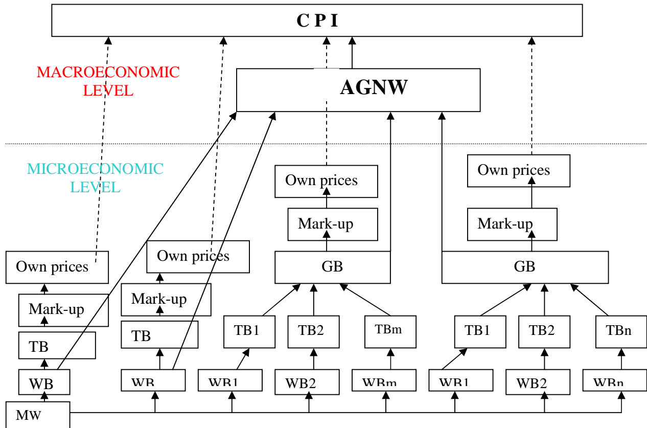
Fig 2. Structure of Fuzzy sets Model.
