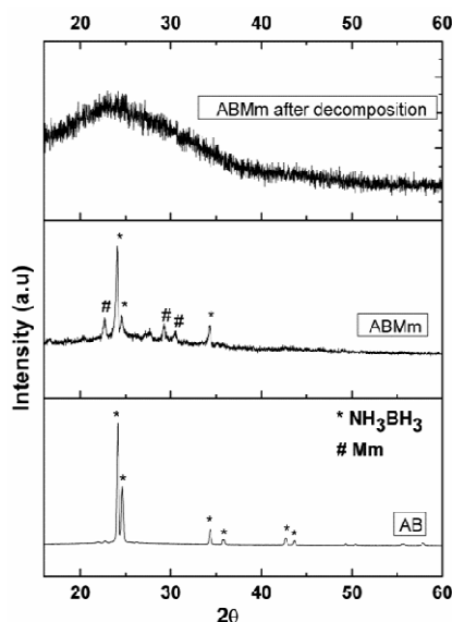
Figure 1: XRD pattern of AB ABMm and ABMmafter decomposition
