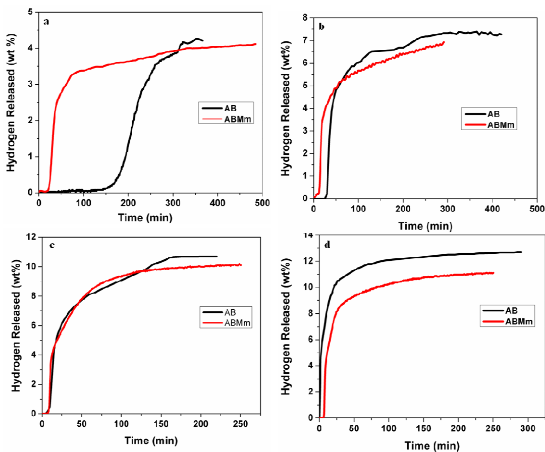
Figure-4 Isothermal decomposition plots of AB and ABMm at (a)90°C, (b)100°C, (c)110°C and (d)150°C
