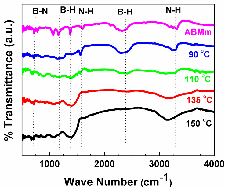
Figure 2: FTIR Spectrum of AB Mm before and after decomposition at different temperature
