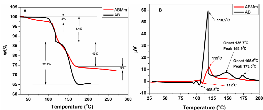
Figure 3: TGA (left) and DTA (right) plots for AB and ABMm
