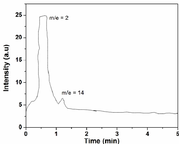
Figure 5 : Chromatograph of gas Evolved of isothermal decomposition of ABMm
